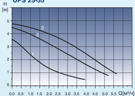
UPS 25-55
