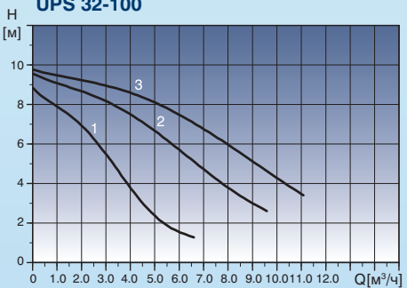
UPS 32-100
