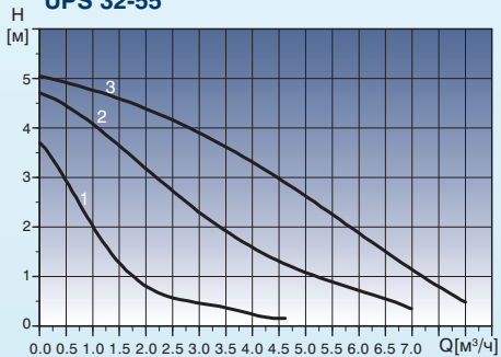
UPS 32-55
